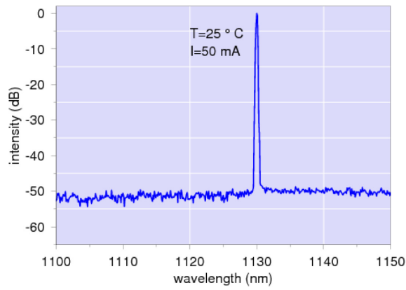
Room Temperature CW Spectrum at 1130nm
